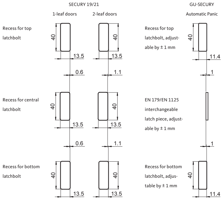
Fig. 4: Approved striker shapes
